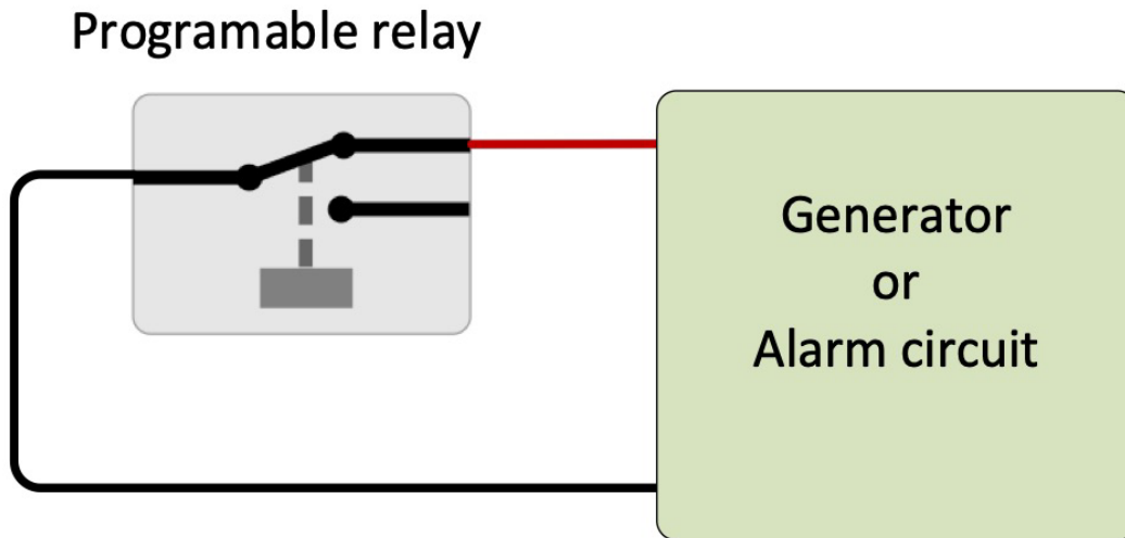
Figure 2. Programmable relay wired to operate as a potential free contact switch
