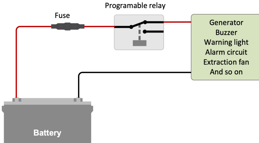
Figure 1. Programmable relay wired to operate a load
